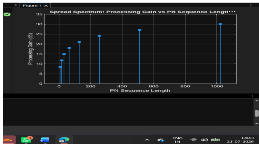
Fig. Processing Gain versus PN Sequence Length
